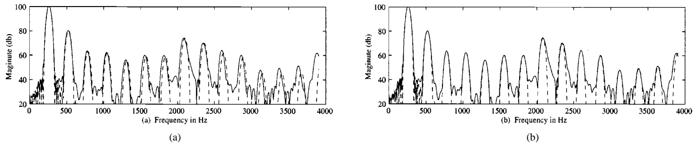
Fig. 1. (a) Original (continuous line) and synthetic (dashed line) magnitude spectra using the initial pitch estimation. (b) Original (continuous line) and synthetic (dashed line) magnitude spectra using the refined pitch value.
