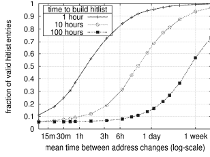
Fig. 11. Effect of NASR on hitlist decay
