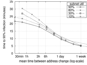
Fig. 12. Effect of NASR vs. subnet usage density
