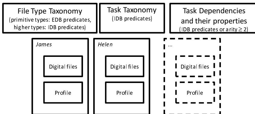
Fig. 1. Logical partitioning
