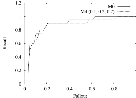
Figure 5: The Recall/Fallout curve of (m_0) and (m_4) on CIDOC CRM
