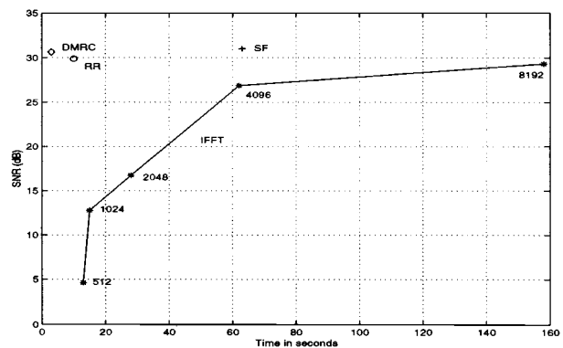
Fig. 1. Comparing the four methods for the generation of a harmonic signal. SF (+), FFT (*), RR(o), DMRC( \diamond ).
