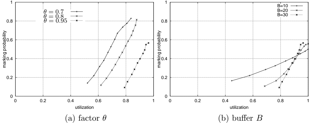
Fig. 10. Effect of the virtual queue factor \theta and the buffer size (single link). C = 10 Mbps, RTT = 200 msec, \bar{w}_{inc} = 1 and 6, \bar{w}_{dec} = 1 , \bar{\kappa} = 0.5 .
