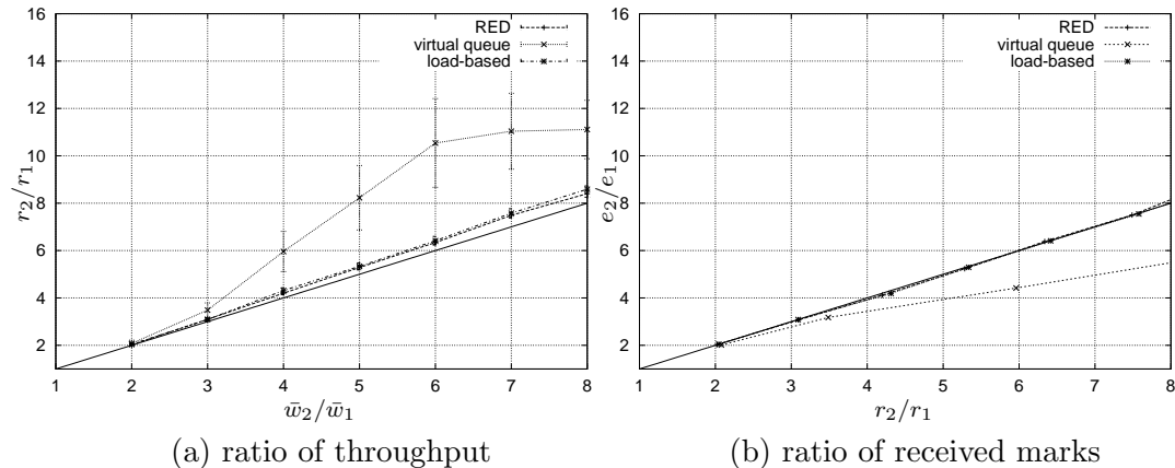
Fig. 3. Service differentiation using proportional increase WTP (single link). \bar{\kappa} = 0.5 . C = 10 Mbps, B = 30 pkts, RTT = 200 ms, N = 10 . RED: min_{th} = 5 , max_{th} = 15 , max_p = 0.1 , w_q = 0.002 . VQ: \theta = 0.95 . LB: t_{avg} = 0.5 s, \rho_0 = 0.6 , \alpha = 0.71 .
