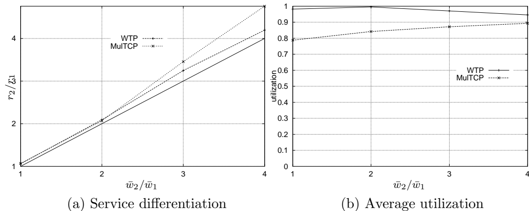
Fig. 11. Comparison of WTP and MultTCP (single link). WTP: \bar{\kappa} = 0.5 , C = 10 Mbps, RTT = 200 msec, N = 10 . RED Marking: min_{th} = 5 , max_{th} = 15 , max_p = 0.1 , w_q = 0.002 .
