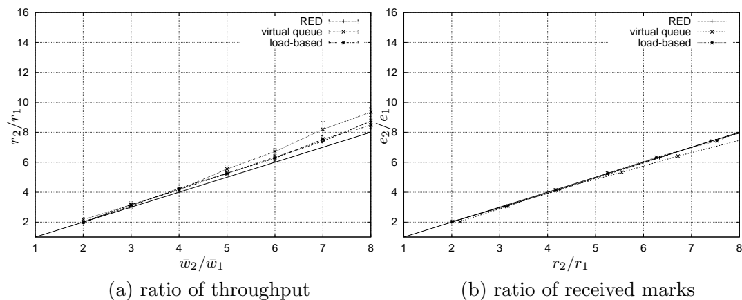
Fig. 4. Service differentiation using inversely proportional decrease WTP (single link). \bar{\kappa} = 0.5 . C = 10 Mbps, B = 30 pkts, RTT = 200 ms, N = 10 . RED: min_{th} = 5 , max_{th} = 15 , max_p = 0.1 , w_q = 0.002 . VQ: \theta = 0.95 . LB: t_{avg} = 0.5 s, \rho_0 = 0.6 , \alpha = 0.71 .
