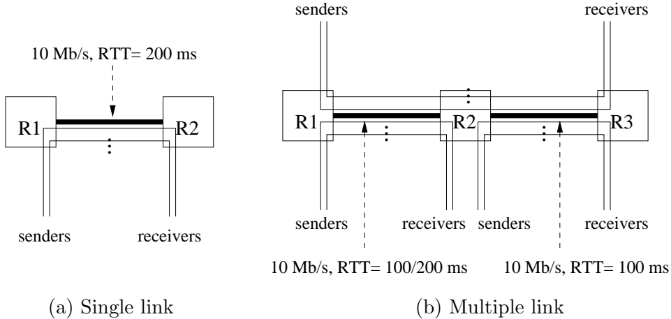
Fig. 2. Network topologies used in the simulation experiments.
