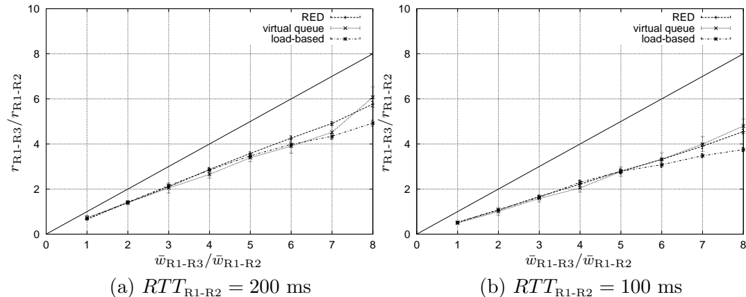
Fig. 5. Service differentiation for different RTT's (multiple link, proportional increase WTP). \bar{\kappa} = 0.5 . C_{R1-R2} = C_{R2-R3} = 10 Mbps, B_{R1-R2} = B_{R2-R3} = 30 pkts, RTT_{R2-R3} = 100 ms, N_{R1-R2} = N_{R1-R3} = 5 , N_{R2-R3} = 0 . RED: min_{th} = 5 , max_{th} = 15 , max_p = 0.1 , w_q = 0.002 . VQ: \theta = 0.95 . LB: t_{avg} = 0.5 s, \rho_0 = 0.6 , \alpha = 0.71 .
