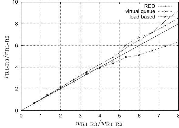
Fig. 6. Throughput ratio as a function of willingness-to-pay ratio (multiple link, proportional increase WTP). \bar{\kappa} = 0.5 . C_{R1-R2} = C_{R2-R3} = 10 Mbps, B_{R1-R2} = B_{R2-R3} = 30 pkts, RTT_{R1-R2} = 200 ms, RTT_{R2-R3} = 100 ms, N_{R1-R2} = N_{R1-R3} = 5 , N_{R2-R3} = 0 . RED: min_{th} = 5 , max_{th} = 15 , max_p = 0.1 , w_q = 0.002 . VQ: \theta = 0.95 . LB: t_{avg} = 0.5 s, \rho_0 = 0.6 , \alpha = 0.71 .
