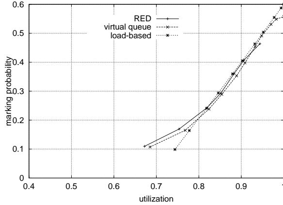
Fig. 9. Marking probability as a function of utilization (single link). \bar{\kappa} = 0.5, \bar{w}_{inc} = 1 and 6, \bar{w}_{dec} = 1 . C = 10 Mbps, B = 30 pkts, RTT = 200 ms. RED: min_{th} = 3, max_{th} = 9, max_p = 0.95, w_q = 0.002 . VQ: \theta = 0.95 . LB: t_{avg} = 0.5 s, \rho_0 = 0.7, \alpha = 2 .
