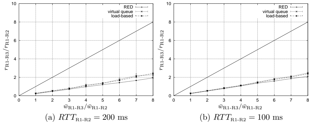
Fig. 7. Service differentiation for different RTT's (multiple link, proportional increase WTP). \bar{\kappa} = 0.5 . C_{R1-R2} = C_{R2-R3} = 10 Mbps, B_{R1-R2} = B_{R2-R3} = 30 pkts, RTT_{R2-R3} = 100 ms, N_{R1-R2} = N_{R1-R3} = N_{R2-R3} = 5 . RED: min_{th} = 5 , max_{th} = 15 , max_p = 0.1 , w_q = 0.002 . VQ: \theta = 0.95 . LB: t_{avg} = 0.5 s, \rho_0 = 0.6 , \alpha = 0.71 .
