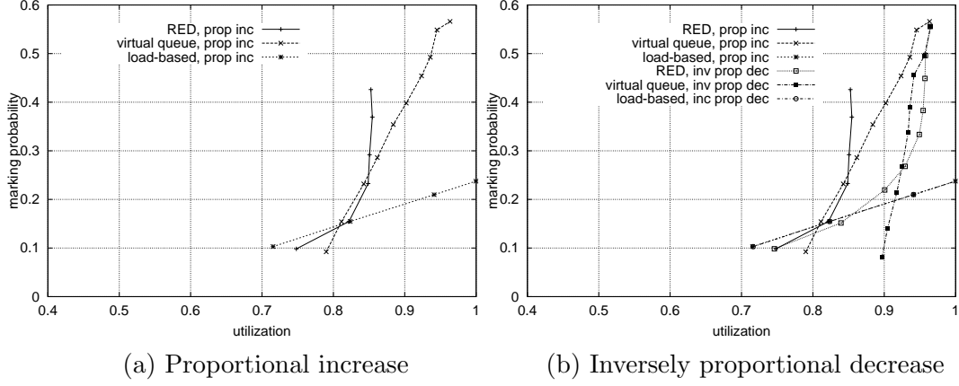
Fig. 8. Marking probability as a function of utilization for proportional increase WTP: \bar{\kappa} = 0.5, \bar{w}_{inc} = 1 and 6, \bar{w}_{dec} = 1 , and inversely proportional decrease WTP: \bar{\kappa} = 0.5, \bar{w}_{inc} = 1, \bar{w}_{dec} = 1 and 6 . C = 10 Mbps, B = 30 pkts, RTT = 200 ms. RED: min_{th} = 2, max_{th} = 6, max_p = 0.1, w_q = 0.02 . VQ: \theta = 0.95 . LB: t_{avg} = 0.5 s, \rho_0 = 0.6, \alpha = 0.71 . (single link)
