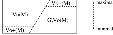
Figure 9: The set relationships of V_o^+(M) and V_o^-(M) .
