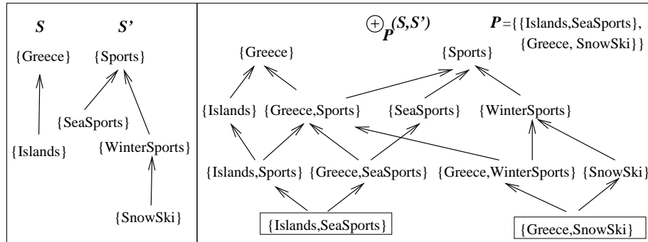
Figure 4: An example of a plus-product , \oplus_P , operation
