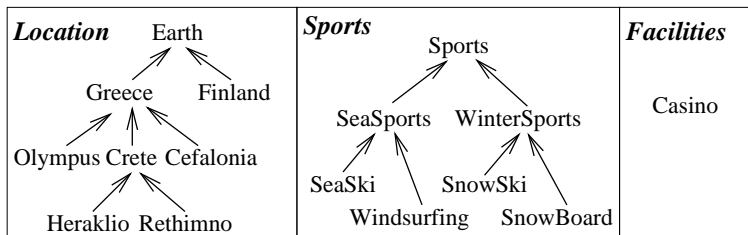
Figure 1: A faceted taxonomy for indexing hotel Web pages
