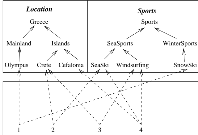
Figure 5: A materialized faceted taxonomy
