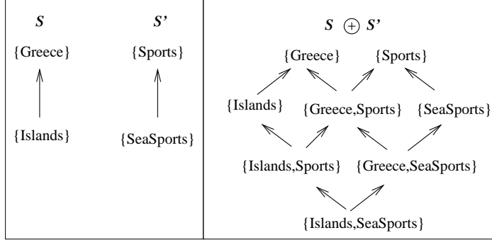
Figure 3: An example of a product \oplus operation
