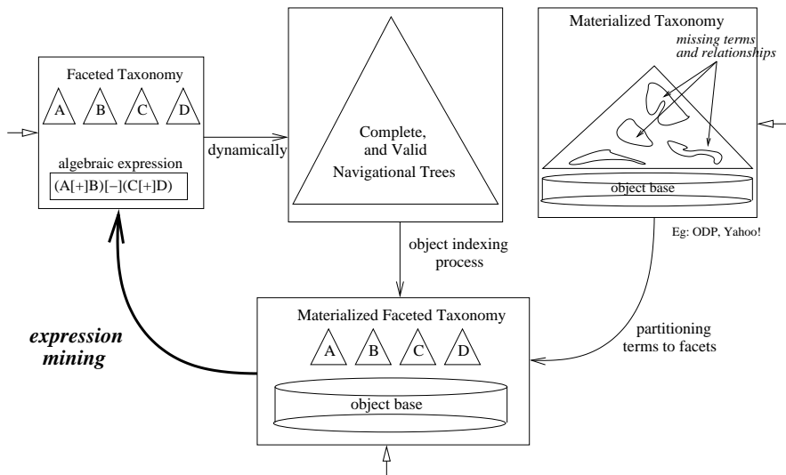
Figure 2: Some application scenarios of expression mining
