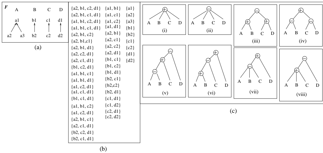
Figure 7: An example of shortest expression mining
