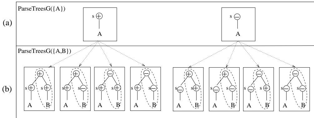
Figure 8: All possible parse trees for \{A\} and \{A, B\}
