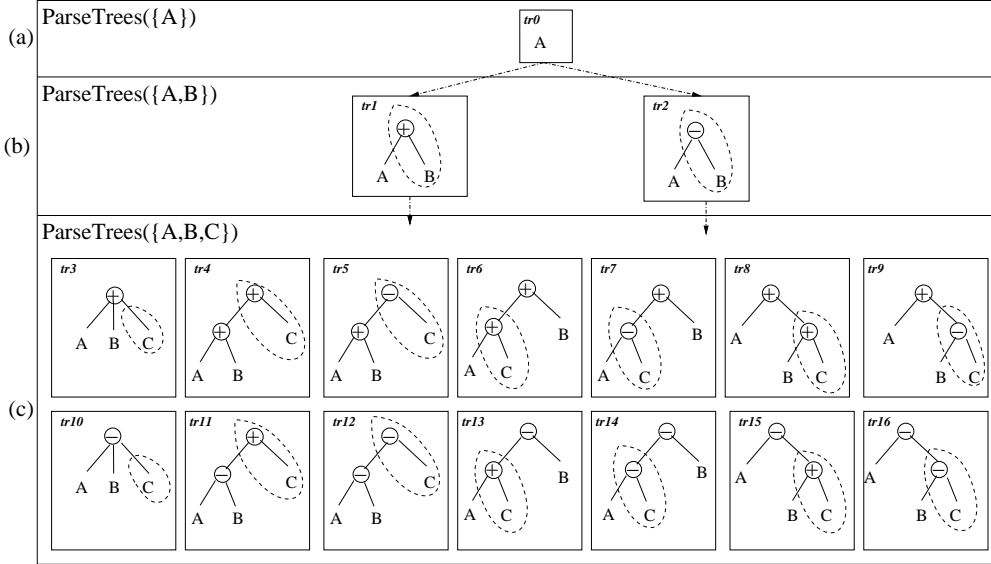
Figure 6: All possible parse trees for \{A\} , \{A, B\} , and \{A, B, C\}
